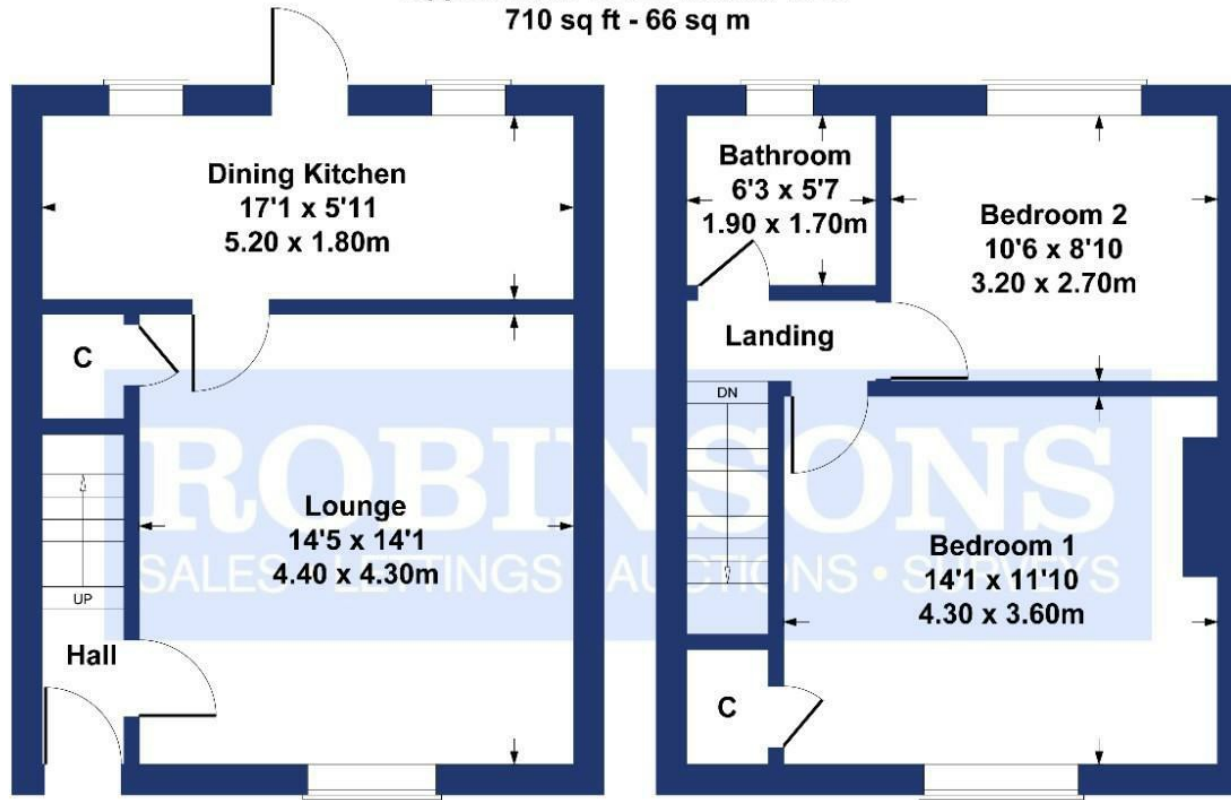
GROUND FLOOR
